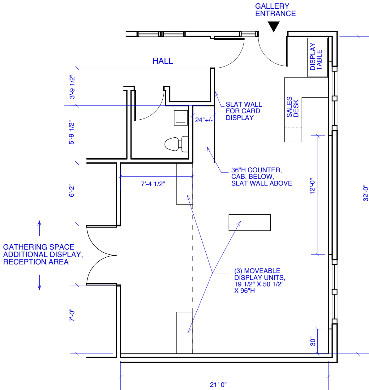
MEETINGHOUSE ARTS GALLERY - FLOOR PLAN
